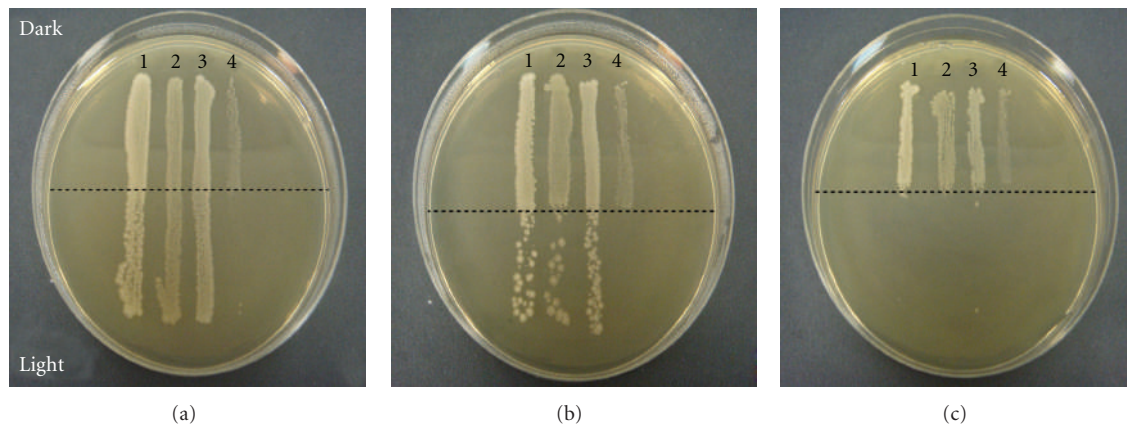
FIGURE 3: Qualitative representation of the bactericidal effect of high-intensity 405 nm light on (1) E. coli , (2) S. sonnei , (3) S. enterica , and (4) L. monocytogenes . Plates (a), (b), and (c) demonstrate the inactivating effect of 15, 30, and 45 minutes light exposure, respectively, on streaks of the foodborne pathogenic bacteria, with half of each plate being light exposed and the other half being kept in darkness to provide the equivalent non-light-exposed control.
